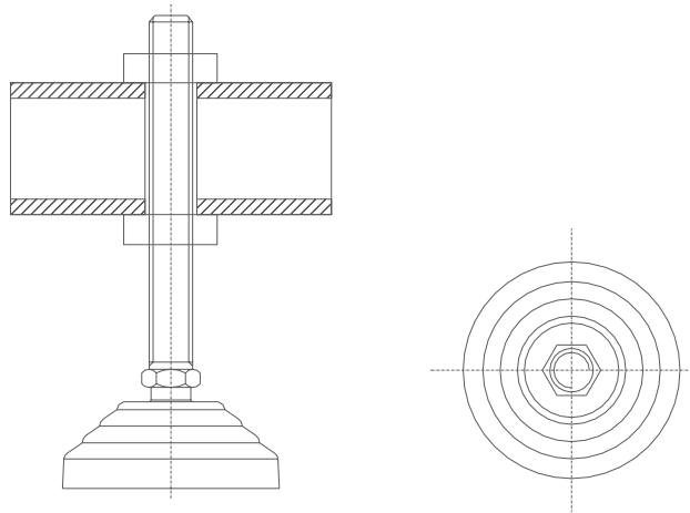
Detail of regulation support
