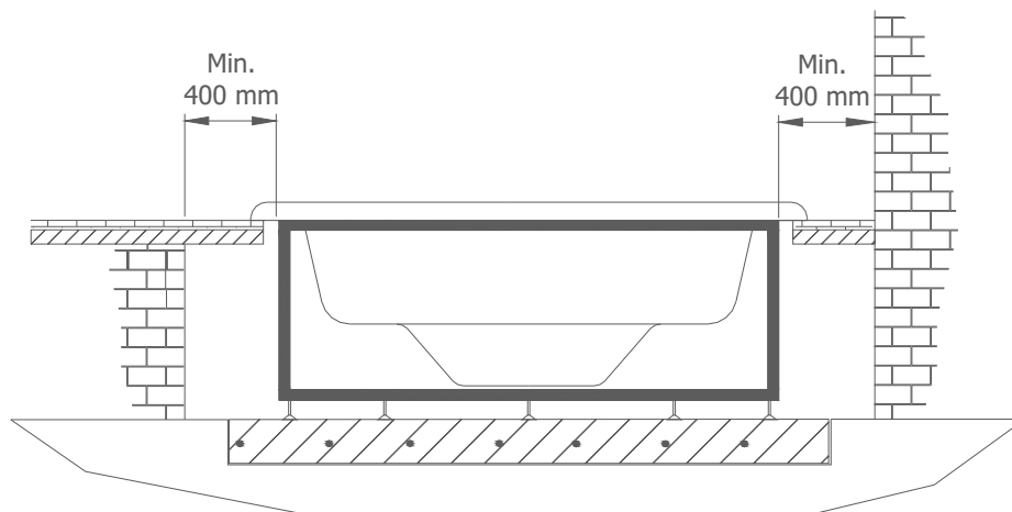
Diagram of minimum distance around the Spa
