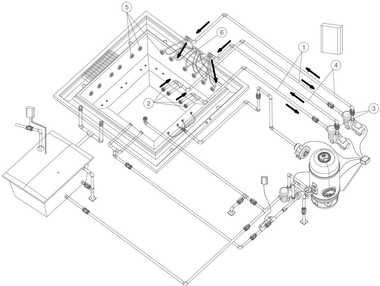
General diagram of water Spa Massage
