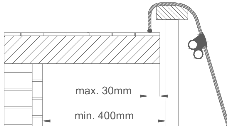
Detail of Lip Sealing
