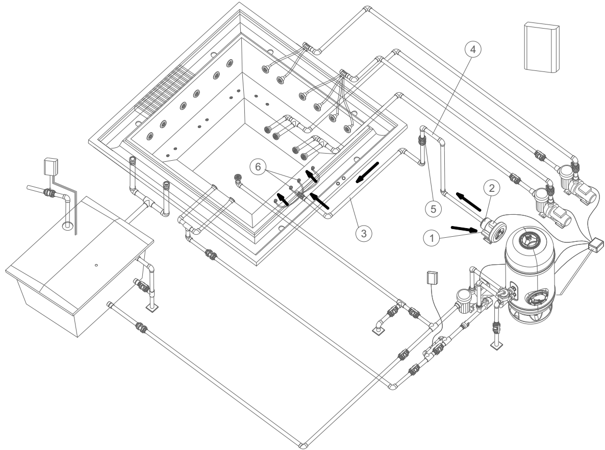
General diagram of Air Spa Massage
