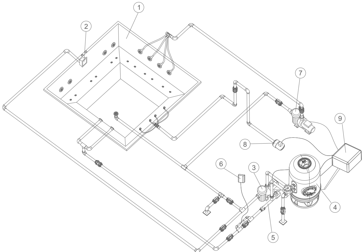
General diagram of Spa with Skimmer
